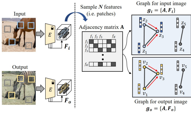
Figure 3: The construction of graphs g_o, g_i with shared adjacency matrix A . Each graph extracts l -hop features Z, V from the given node F_i, F_o .
